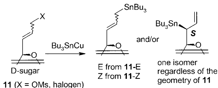
Figure 2: Regioselectivity of formation of sugar allyltins.
