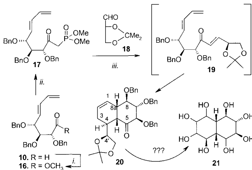
Scheme 3: i. Jones' oxidation, then \text{CH}_2\text{N}_2 ; ii. \text{MeP}(\text{O})(\text{OMe})_2 , \text{BuLi} THF, 15 min, 86%, iii. \text{K}_2\text{CO}_3 , toluene, rt, 18-crown-6, 75%.
