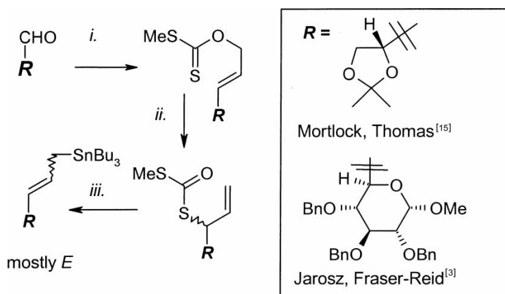
Scheme 2: i. 1. \text{Ph}_3\text{P}=\text{CHCO}_2\text{Me} ; 2. DIBAL-H; 3. \text{NaH}/\text{CS}_2/\text{MeI} ; ii. 80^\circ\text{C} (ref. 15) or 110^\circ\text{C} (ref. 3); iii. \text{Bu}_3\text{SnH} .
