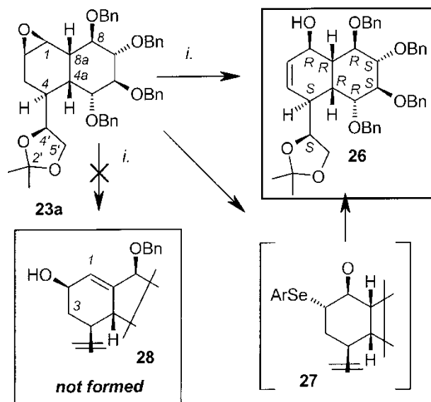
Scheme 4: i. 1. NaBH 4 , EtOH, (PhSe) 2 , 5 min, then 23a reflux 2 h; ii. THF, H 2 O 2 , 0°C to rt, overnight; 93% overall.
