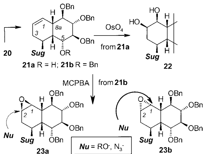
Figure 5: Partial functionalization of decalin precursor 20 .
